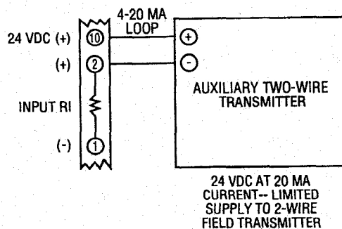
24VDC TWO-WIRE POWER OPTION "O 15"
