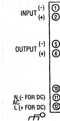
24VDC TWO-WIRE POWER OPTION "O 15"
