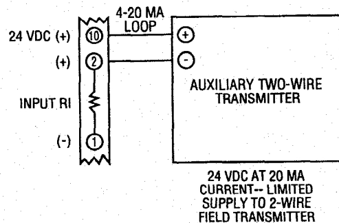
24VDC TWO-WIRE POWER OPTION "O 15"
