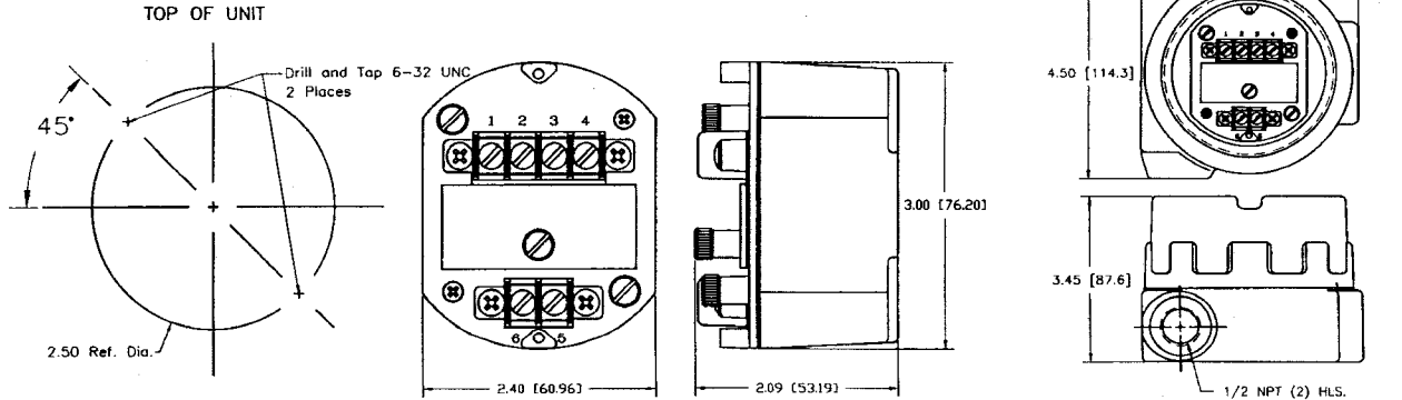
SURFACE MOUNT STANDARD HOUSING
